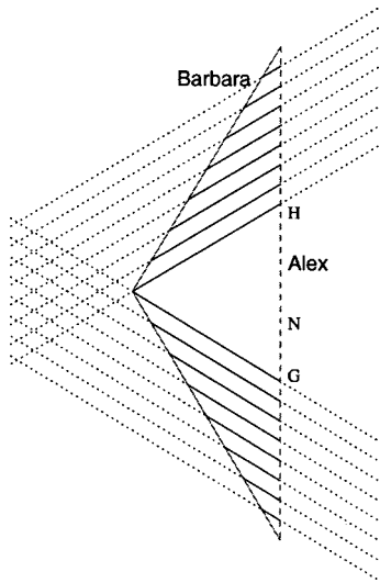
Fig. 1. A typical “textbook illustration” of the hypersurfaces of simultaneity of the traveling twin in the twin paradox.
