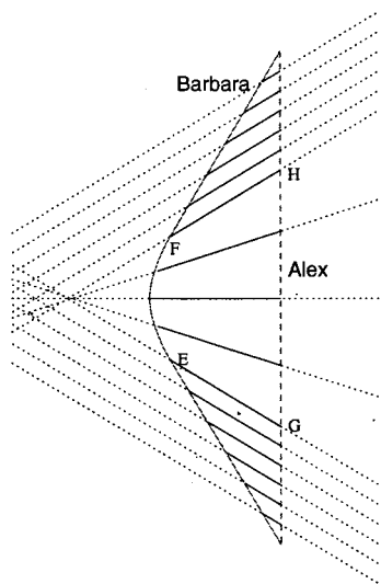
Fig. 2. Another typical “textbook illustration,” in which Barbara’s hypersurfaces of simultaneity “sweep round” from EG to FH during her period of acceleration.
