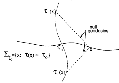
Fig. 3. Schematic of the definition of “radar time” \tau(x) .
