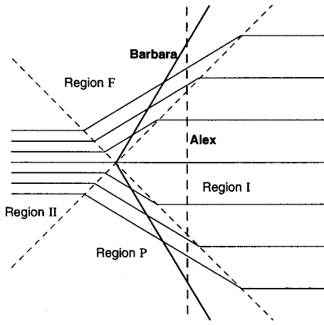
Fig. 5. Hypersurfaces of simultaneity of the traveling twin in the “immediate turn-around” case.
