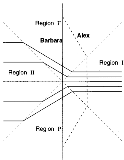
Fig. 9. Alex's hypersurfaces of simultaneity, as described in Barbara's (\tau, \rho) coordinates, for the "immediate turn-around" case.
