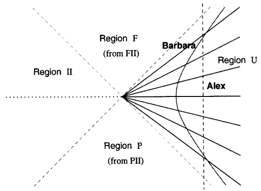
Fig. 7. Hypersurfaces of simultaneity of a uniformly accelerating observer.
