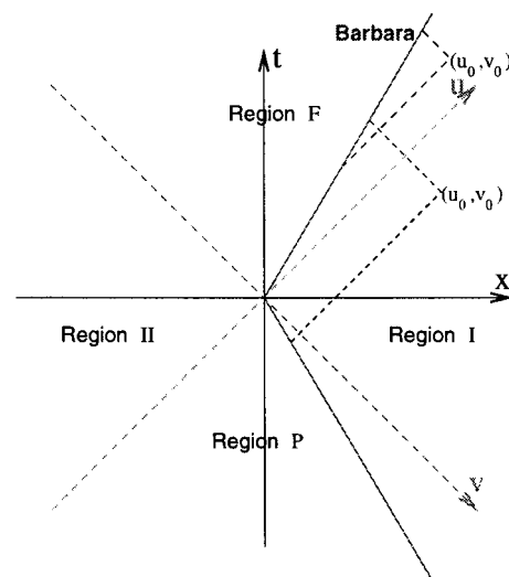
Fig. 4. The traveling twin in the “immediate turn-around” case.
