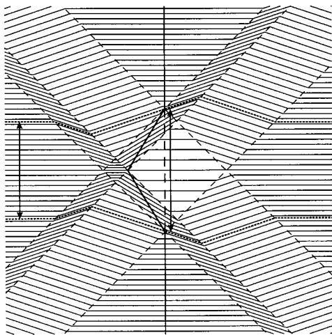
Fig. 10. Hypersurfaces of simultaneity of the traveling twin in the more realistic case, in which their trajectories coincide before and after the journey.
