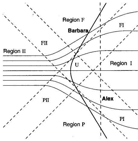
Fig. 6. Hypersurfaces of simultaneity of the traveling twin in the “gradual turn-around” case.
