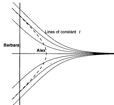
Fig. 8. Alex’s hypersurfaces of simultaneity as described in Barbara’s (\tau, \rho) coordinates, for the “uniformly accelerating” case.
